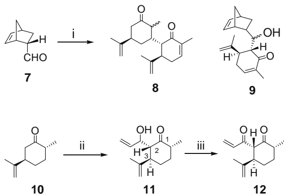
Scheme 2. Reagents and conditions: (i) LDA, THF-HMPA, -100\text{ }^{\circ}\text{C} , R -carvone, 15 min, 40%; (ii) LDA, THF, -78\text{ }^{\circ}\text{C} , acrolein, 10 min, 70%; (iii) DMP, \text{CH}_2\text{Cl}_2 , 1 h, 92%.
