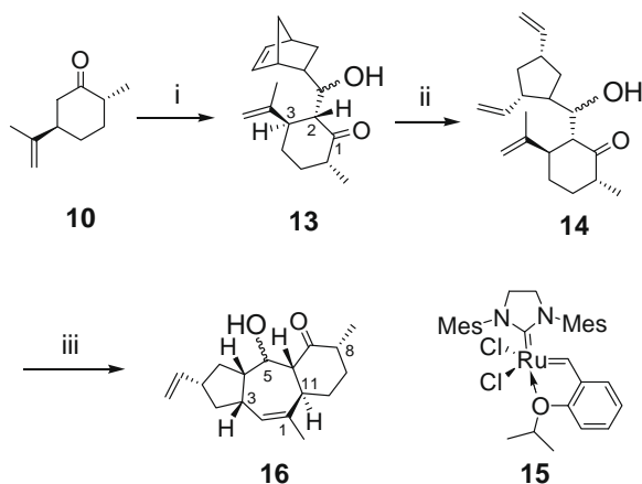
Scheme 3. Reagents and conditions: (i) LDA, THF-HMPA, -100\text{ }^{\circ}\text{C} , 7 , 15 min, 70%; (ii) 5 mol % Grubbs' I, \text{CH}_2=\text{CH}_2 , \text{CH}_2\text{Cl}_2 , 6 h, quant.; (iii) 30 mol % of cat. 15 , toluene, 110\text{ }^{\circ}\text{C} , 2 h, 45%.
