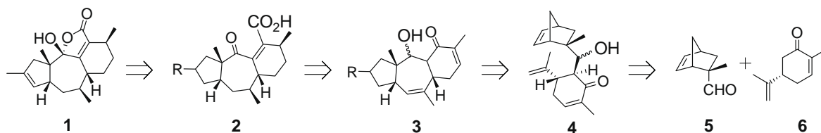
Scheme 1. General retro synthetic analysis.
